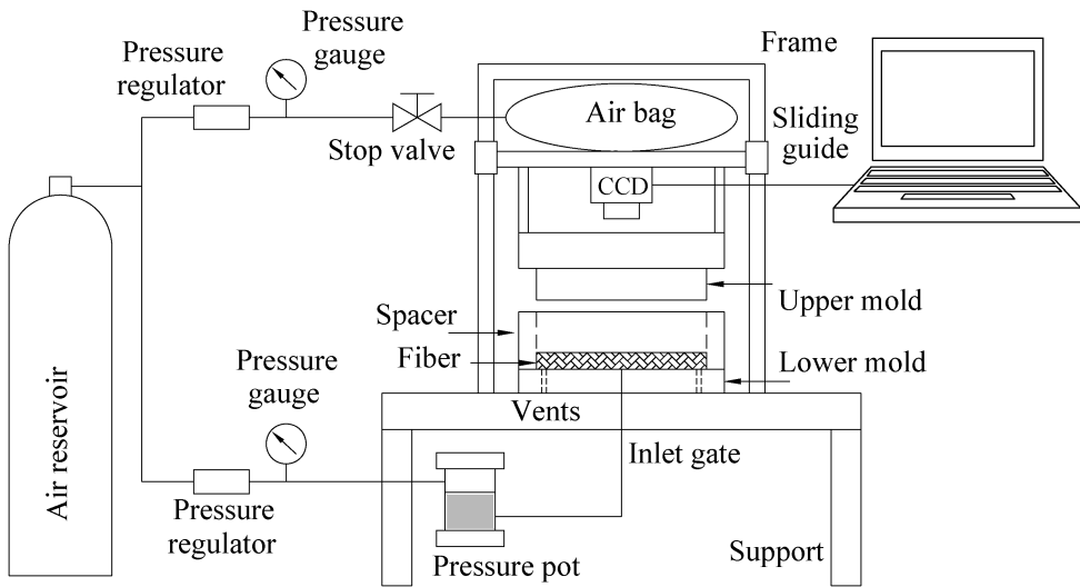
Figure 3. Experimental setup.
