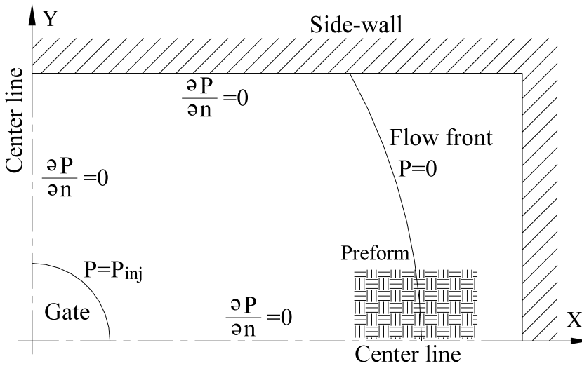
Figure 2. Boundary conditions.
